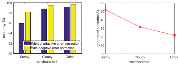
(a) Transmission accuracy. (b) Energy harvesting. Fig. 8. The impact of environment.
