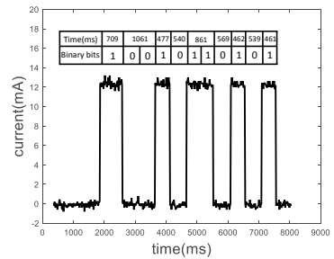
(a) flashlight generated current example
