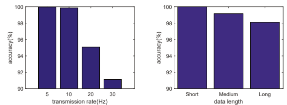
(a) Transmission rate. (b) Data length Fig. 9. The impact of transmission rate and data length.
