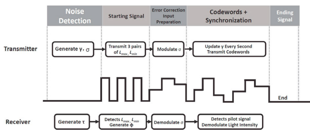
Fig. 3. Transmission process illustration.
