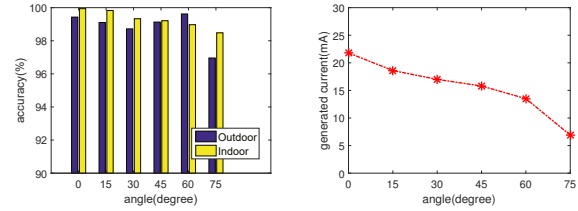
(a) Transmission accuracy. (b) Energy harvesting. Fig. 7. The impact of angle.
