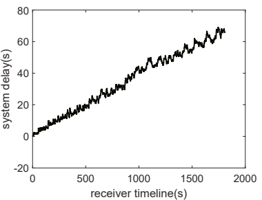
(b) PLL system time difference study
