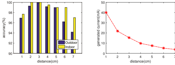
(a) Transmission accuracy. (b) Energy harvesting. Fig. 6. The impact of distance.
